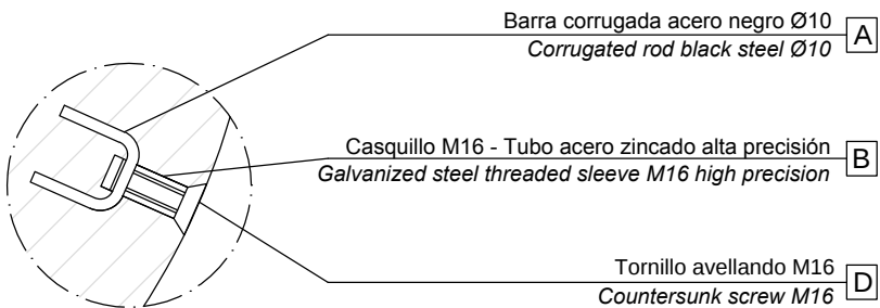
DETALLE M / DETAIL M
