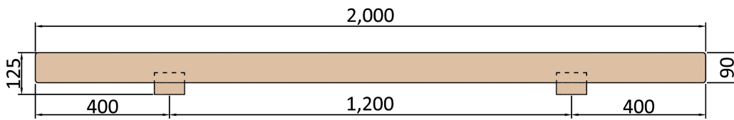
FRONT ELEVATION
