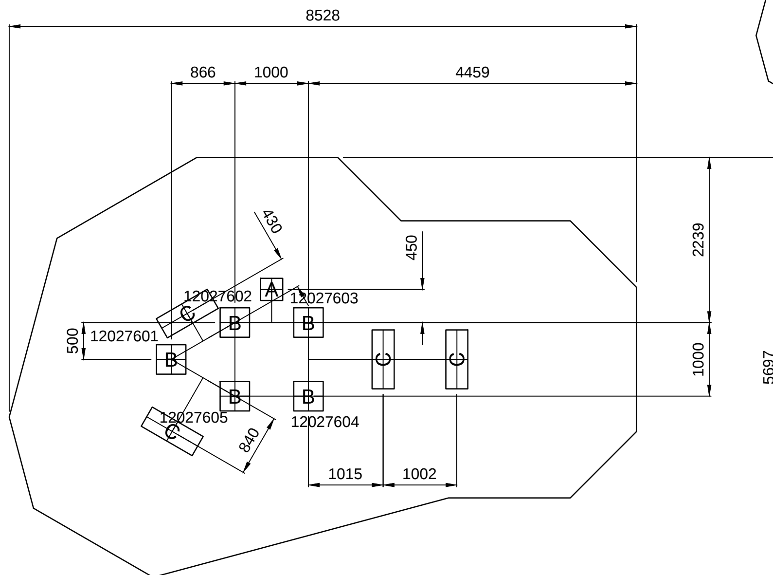
PLAN SCALE 1:100
