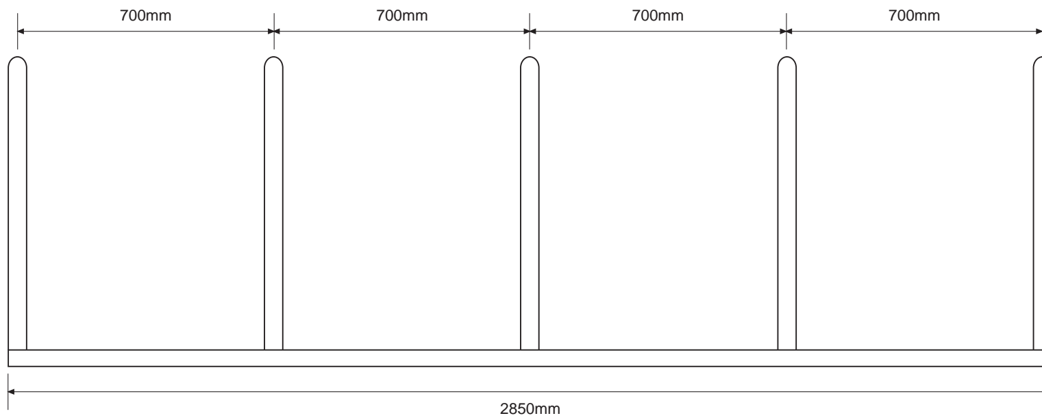
ASF 9009/R5 Mild Steel Floor Mounted
