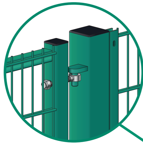
Hinge Detail
