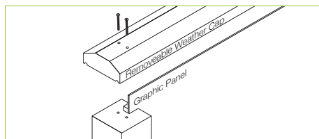
Standard frame assembly
