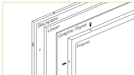
Standard frame assembly
