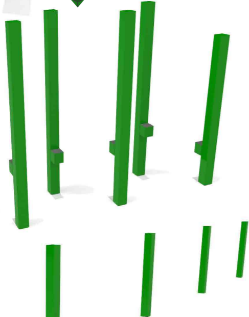
Steel Stilts L 3600 W 540 H 1800mm FFH 590mm
