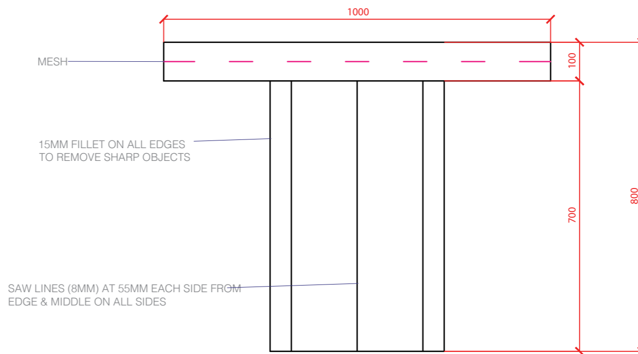
Front View Scale 1:5
