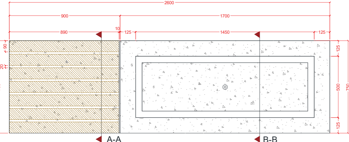
Detail 1: Plan of Planter & Bench
