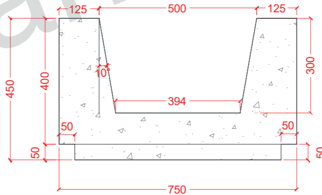
Detail 3: Profile B-B
