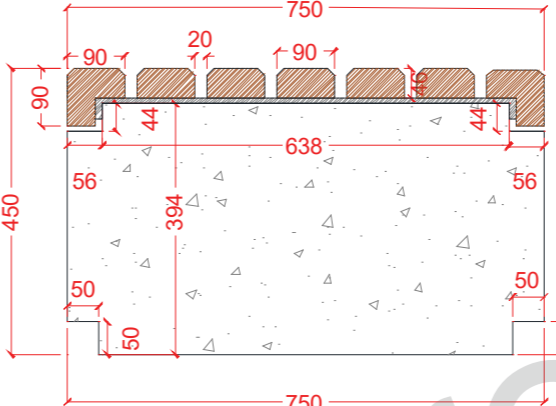
Detail 2: Profile A-A
