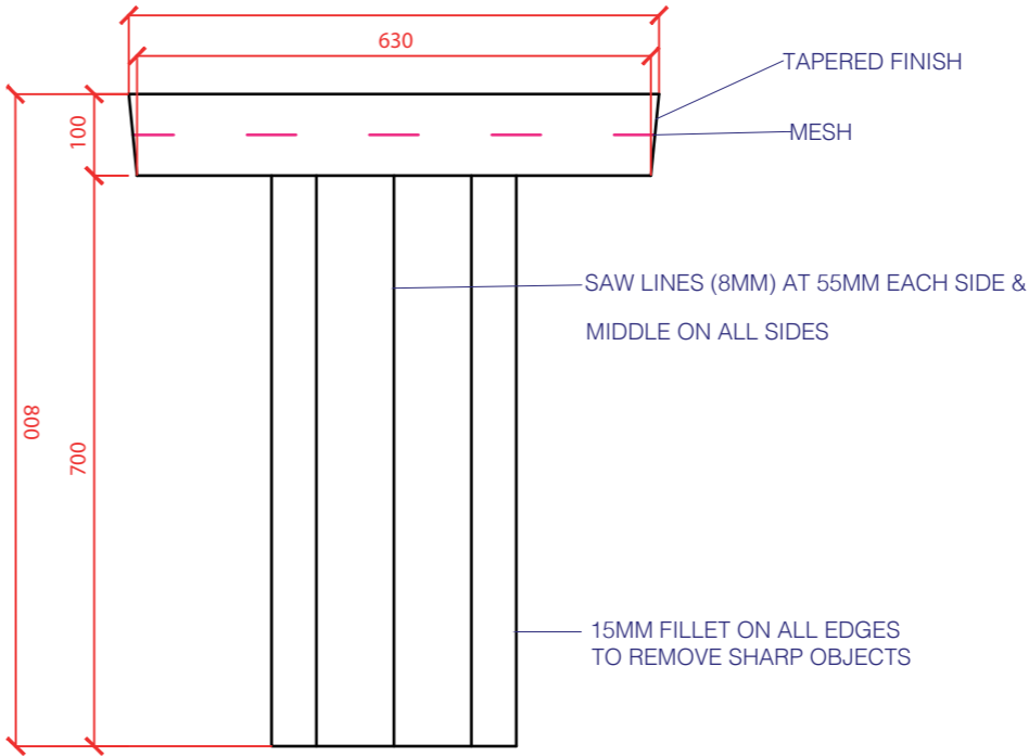
Front View 1:5
