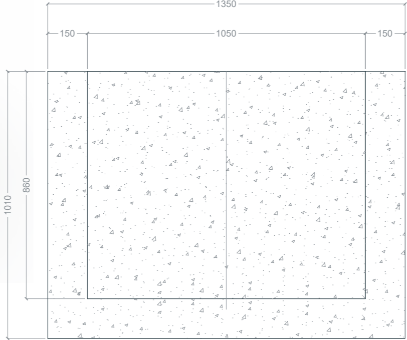
Detail 3: Planter Sectional View
