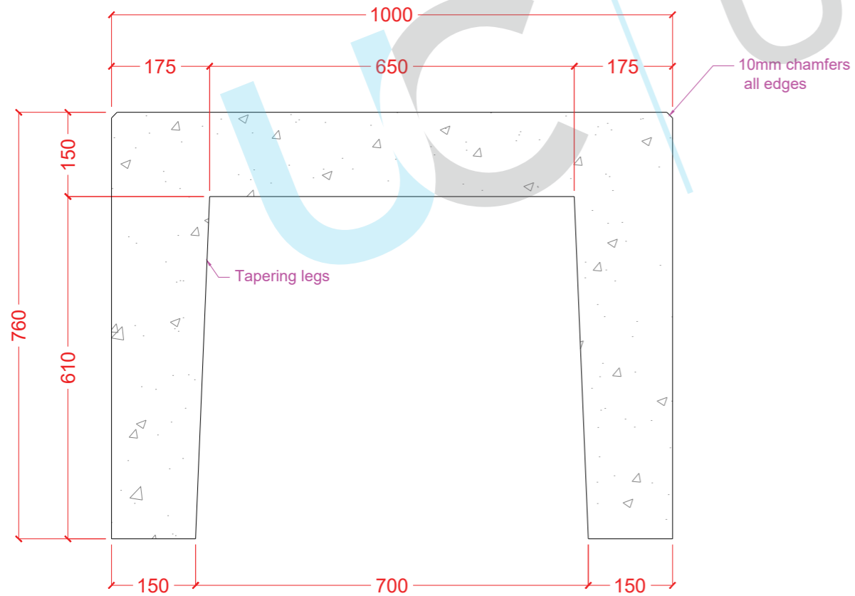
DETAIL 3: SIDE PROFILE CHESS TABLE
