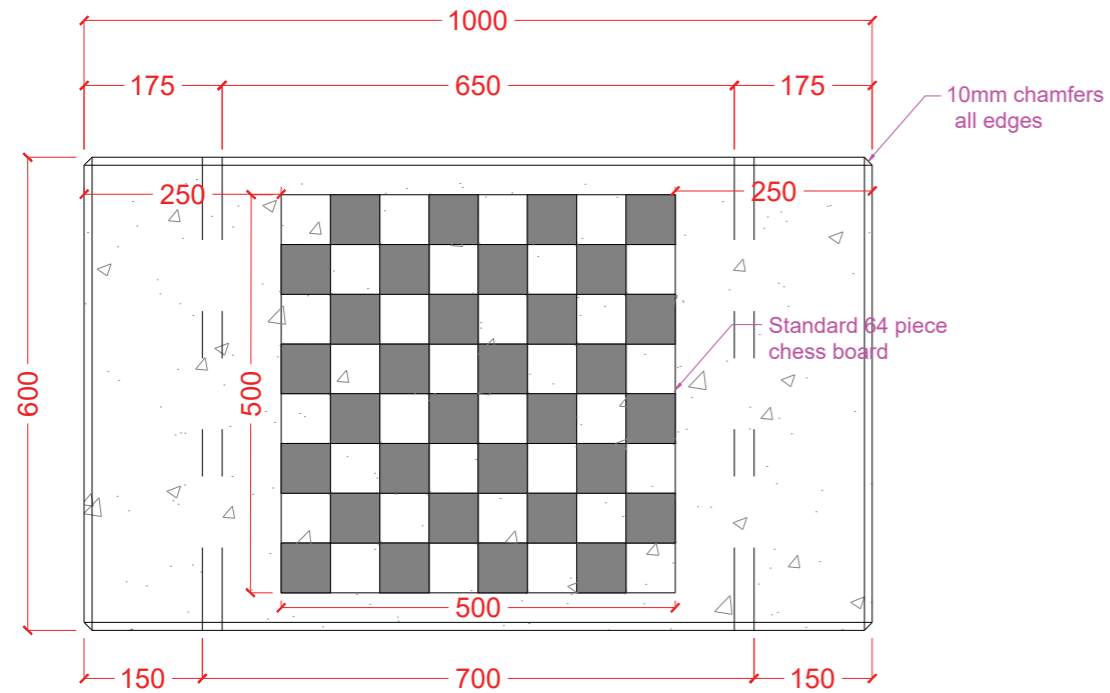
DETAIL 1 : TOP PROFILE CHESS TABLE
