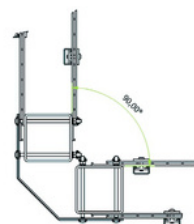
Plan of external corner
