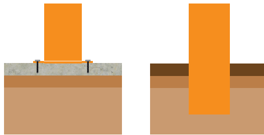
Surface Mounted Baseplate
