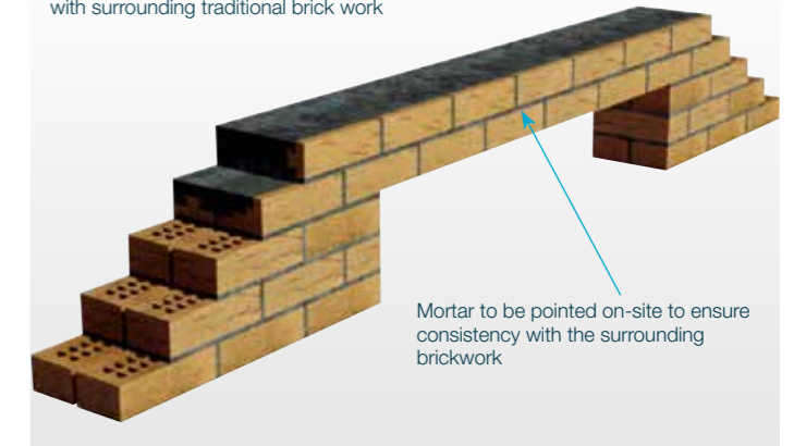
Bearing Lintels
