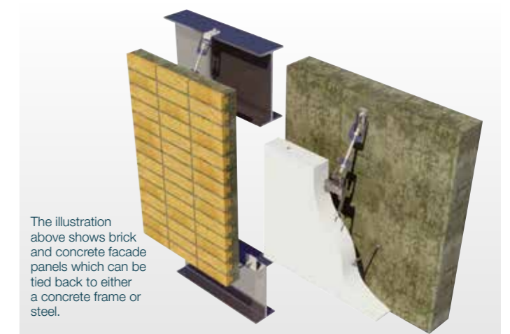
Facade panels
