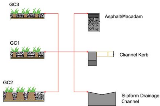
Detail 1 - 6 Scale 1:25
