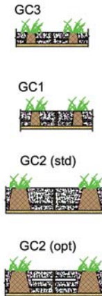
Detail 2
