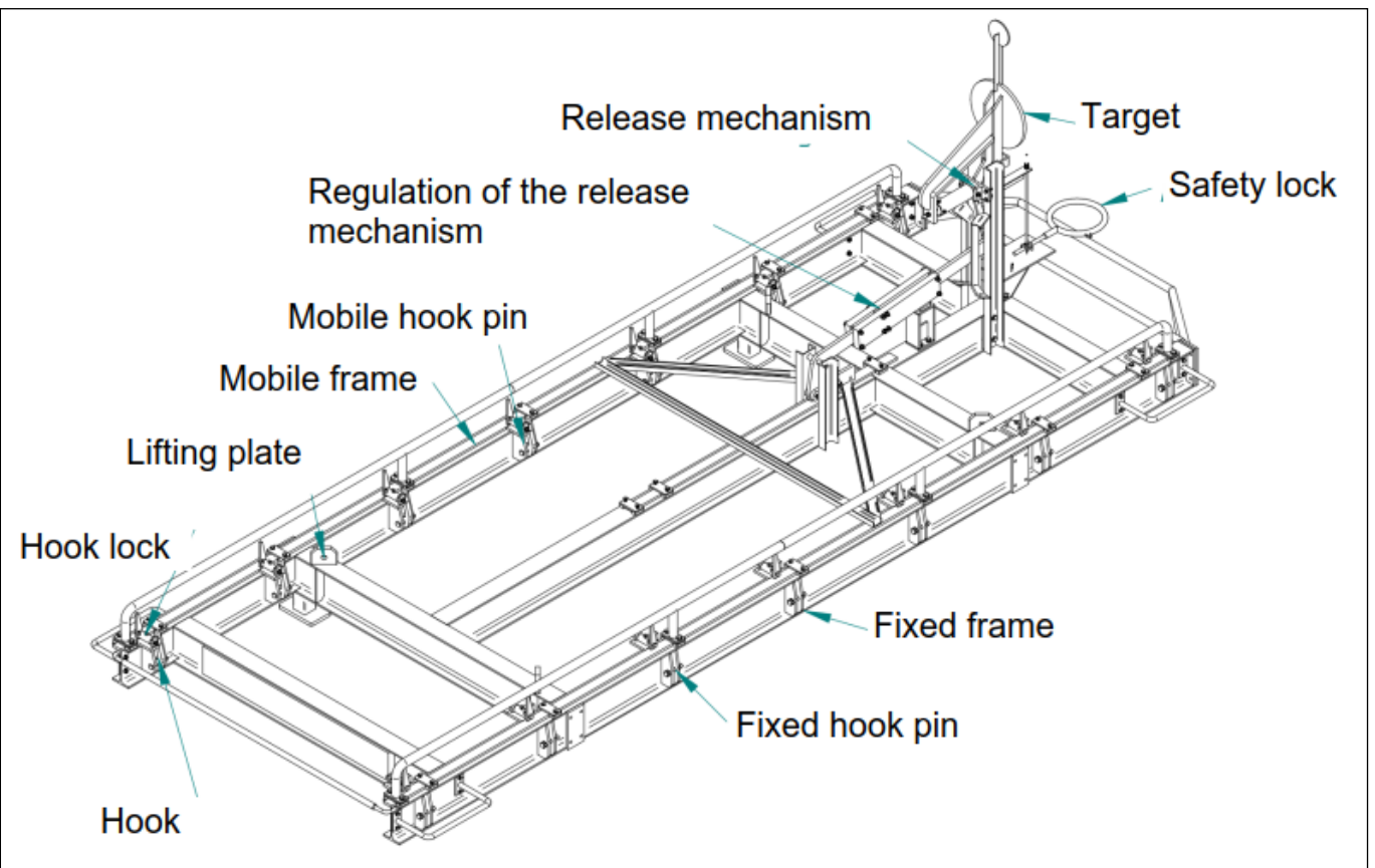
Figure 1: General view and frame components
