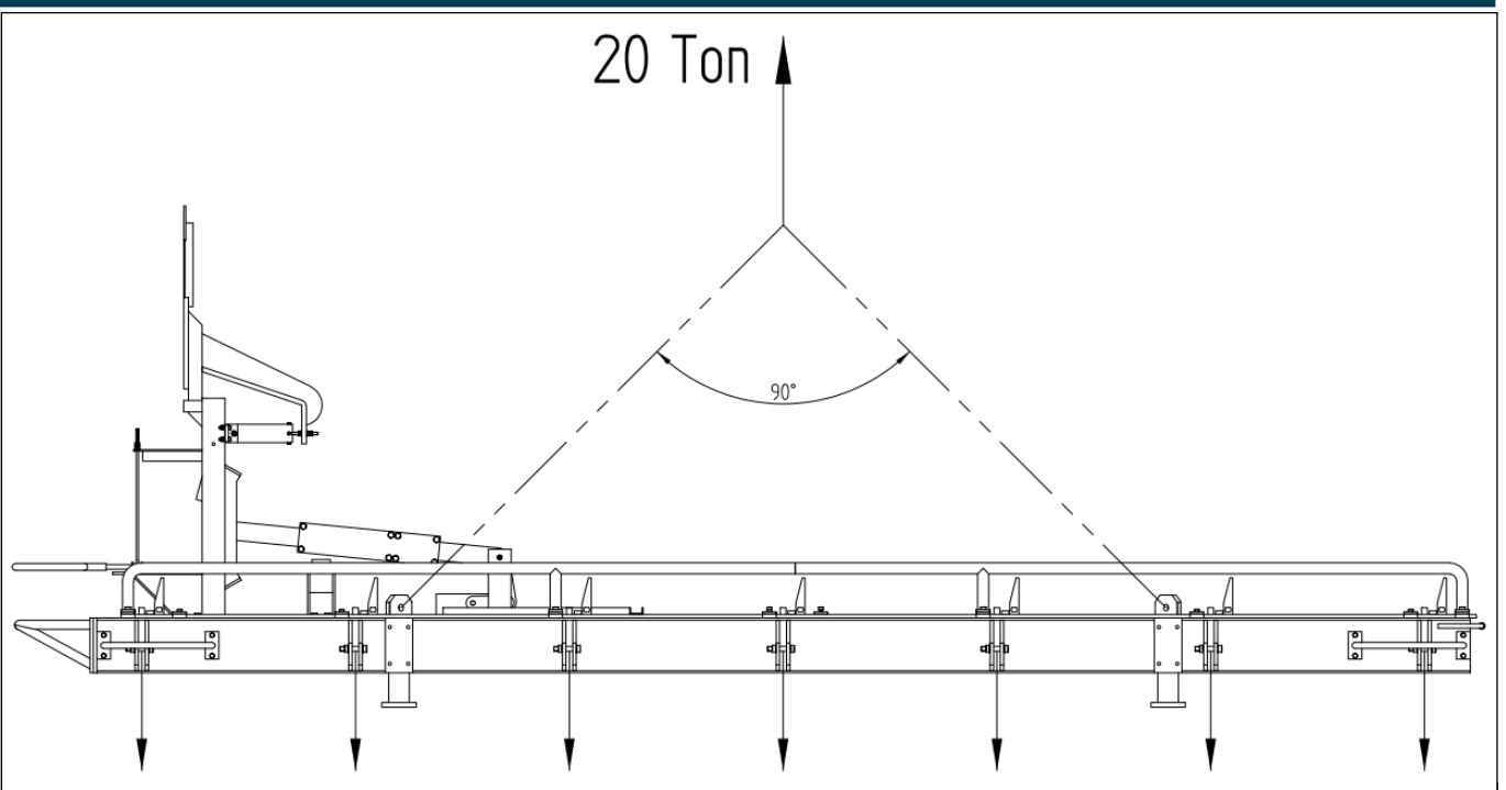
Figure 2: Loading configuration
