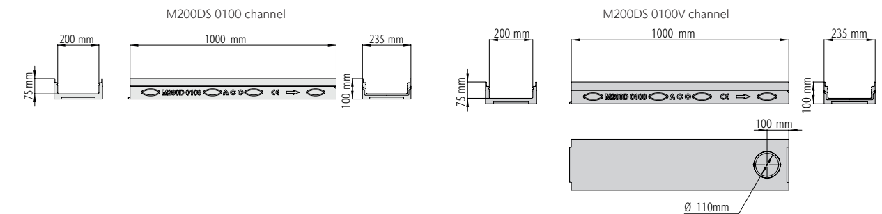
M200DS constant depth channel 0.0 to 20.0
