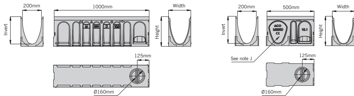
M200DS constant depth channel 0.0 to 20.0
