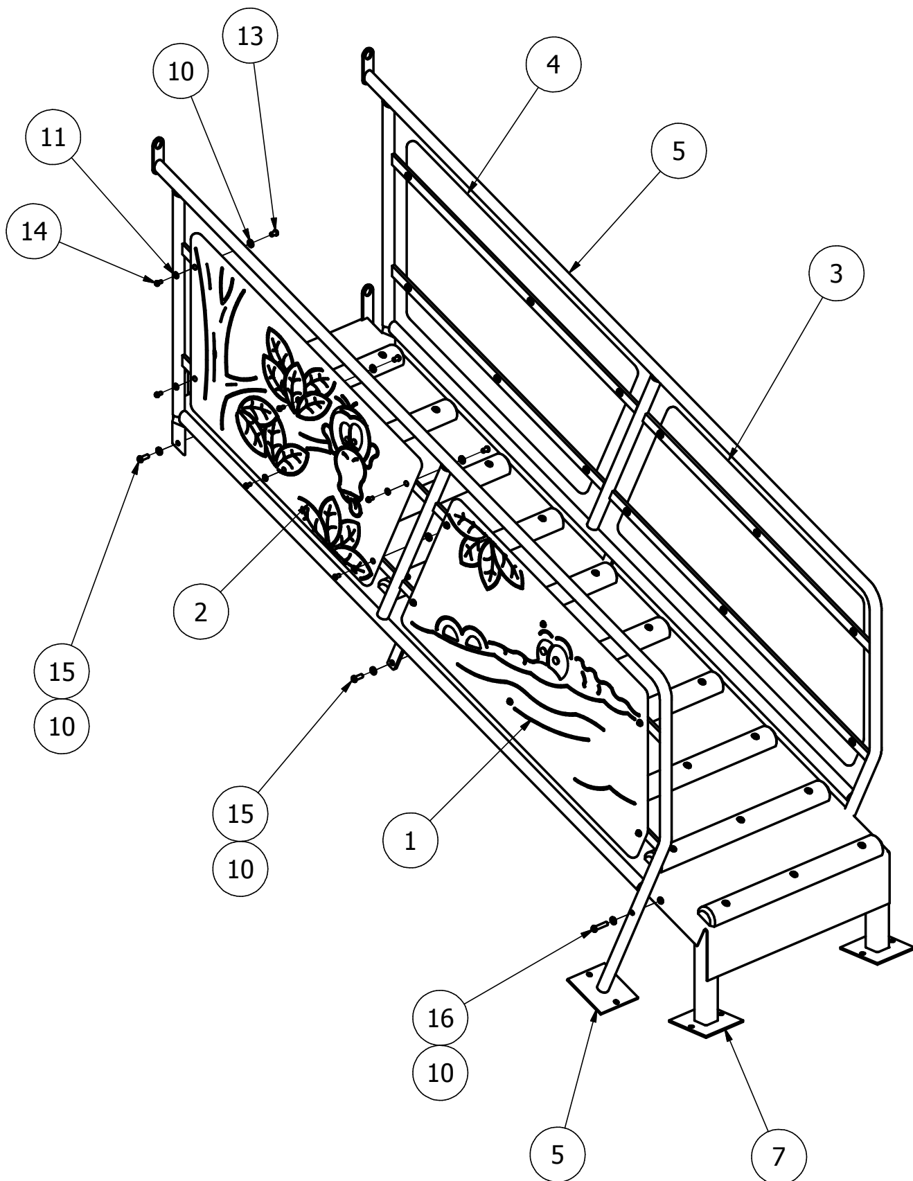
Panels to handrails and handrails to ramp fixing detail
