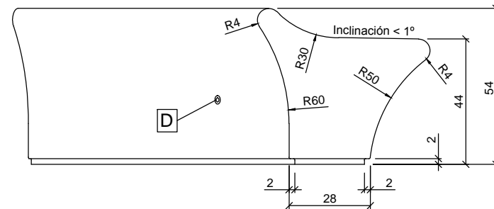
ALZADO / FRONT VIEW
