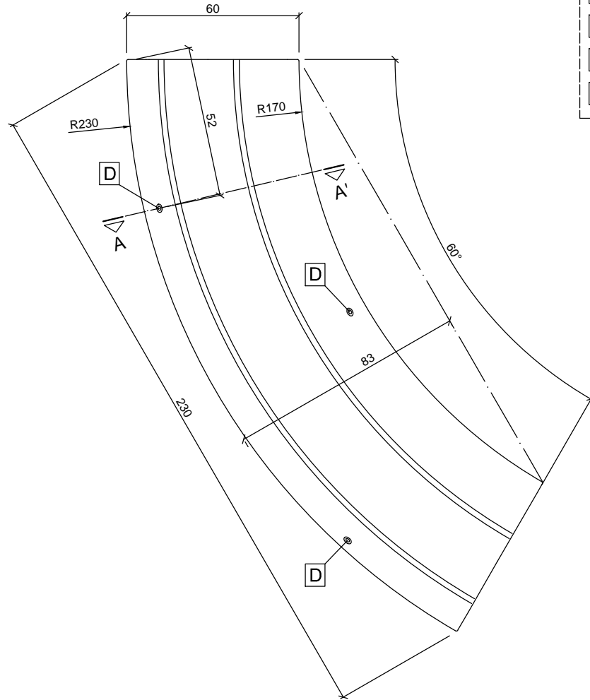
VISTA INFERIOR / BOTTOM VIEW
