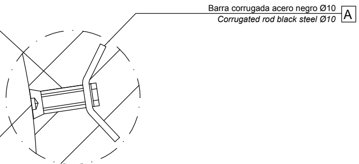
DETALLE M / DETAIL M
