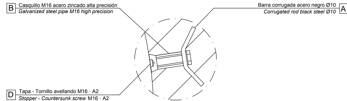
DETALLE M / DETAIL M
