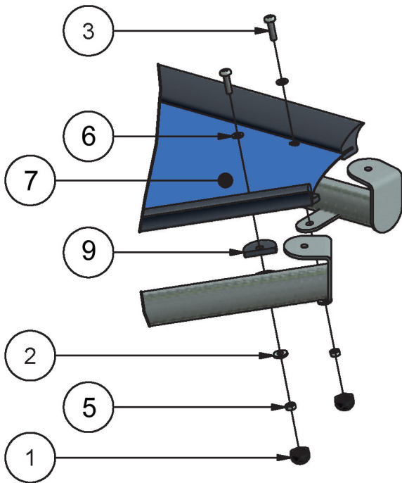
FIXINGS REQUIRED FOR ATTACHING ROOF PANELS TO THE LEGS
