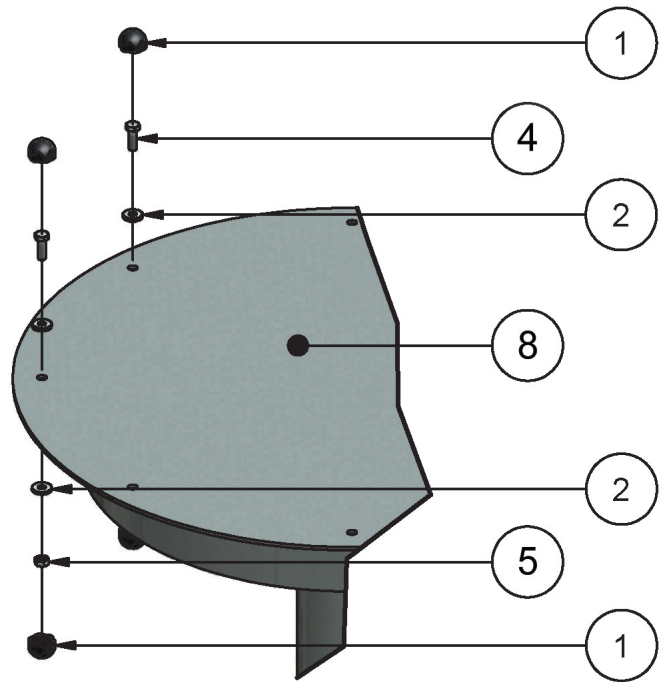
FIXINGS REQUIRED FOR ATTACHING LEGS TO THE CENTRAL POST.
