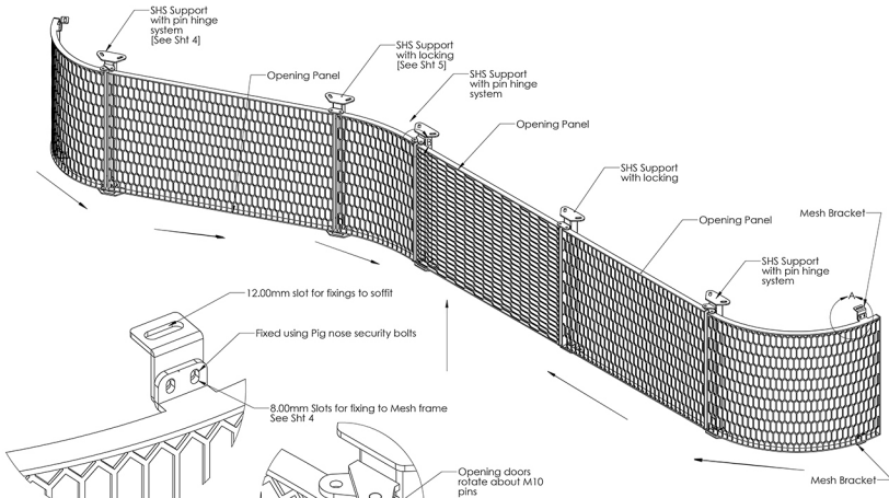
DETAIL A SCALE 1 : 2
