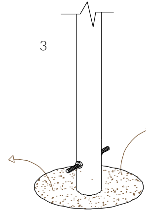
3 Excavate a hole with a 250mm diameter tapering down to 350mm diameter and 450mm depth
